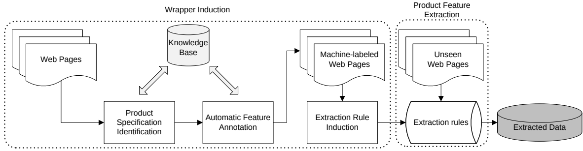
Figure 1: Complete product feature extraction framework.
