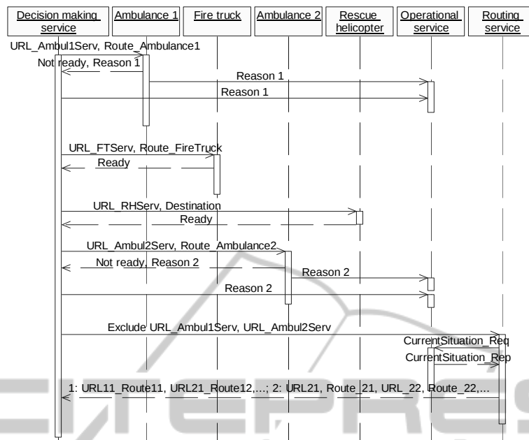
Figure 7: Plan regeneration.
