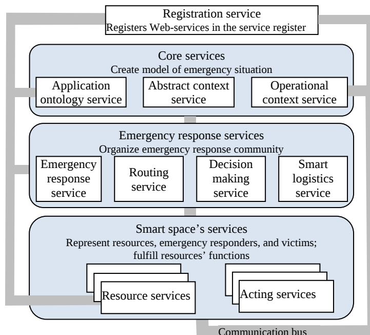
Figure 5: Service-oriented architecture.
