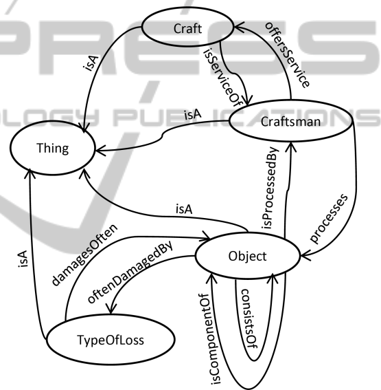
Figure 5: Ontology structure.
