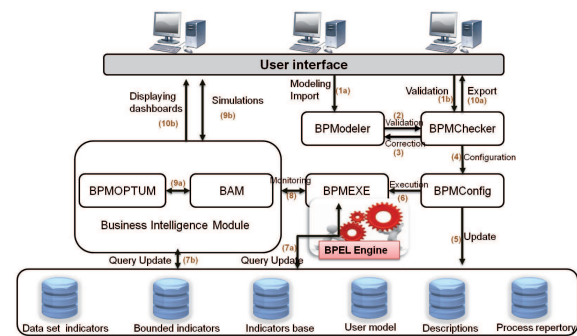
Figure 4: Architecture of our enterprise training processes management system.
