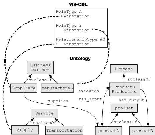
Figure 4: Semantic annotation.
