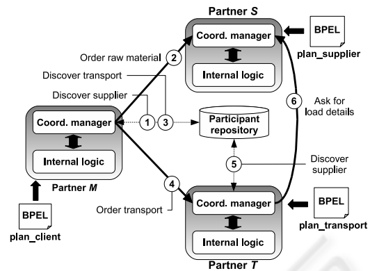
Figure 3: Example execution.
