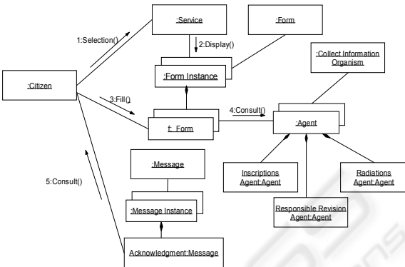
Figure 6.6: Collaboration diagram “Requesting a service”.
