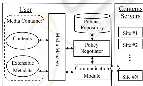
Figure 1: Functional Architecture of the Proposed Metadata System.
