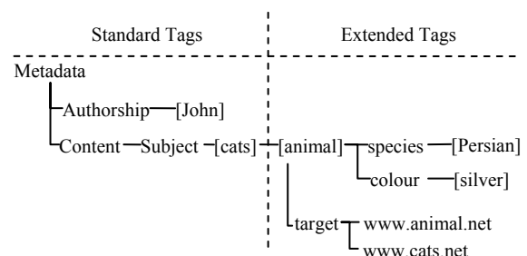
Figure 3: Example of Extending Tag Objects about Cats.
