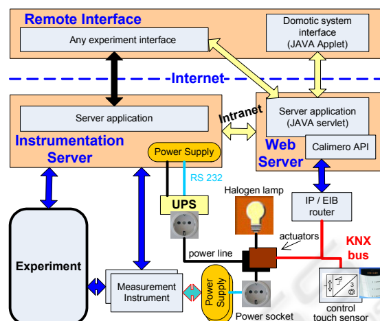
Figure 3: Implemented software architecture to control the KNX/EIB devices.
