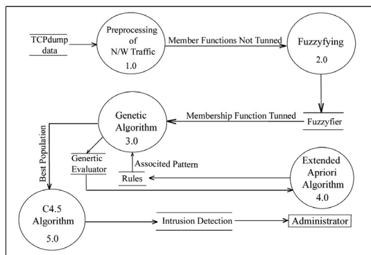
Figure 1: Flow of information of IDS system.
